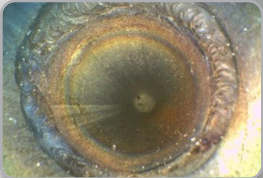
Orbital Weld
